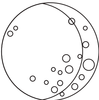
Waxing Crescent
