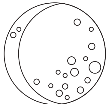
Waxing Gibbous
