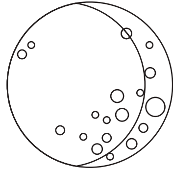
Waning Gibbous
