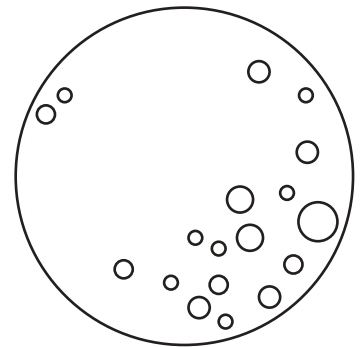
Full Moon
