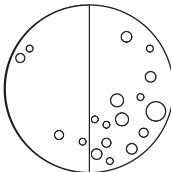
First Quarter
