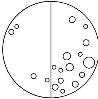
Last Quarter
