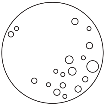
New Moon
