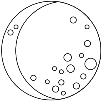
Waning Crescent
