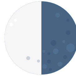
Last Quarter
