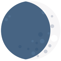
Waxing Crescent
