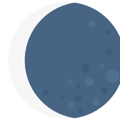
Waning Crescent
