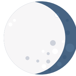
Waning Gibbous
